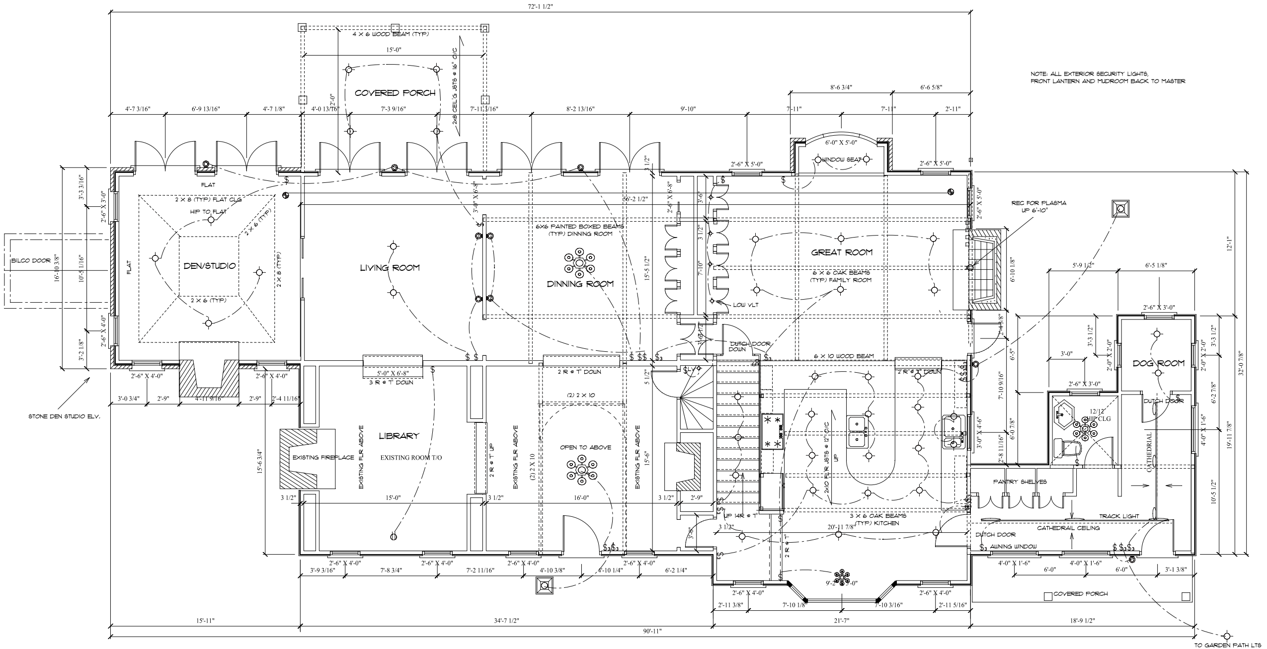
FIRST FLR ELEC PLAN SCALE 1/8" = 1'-0"
