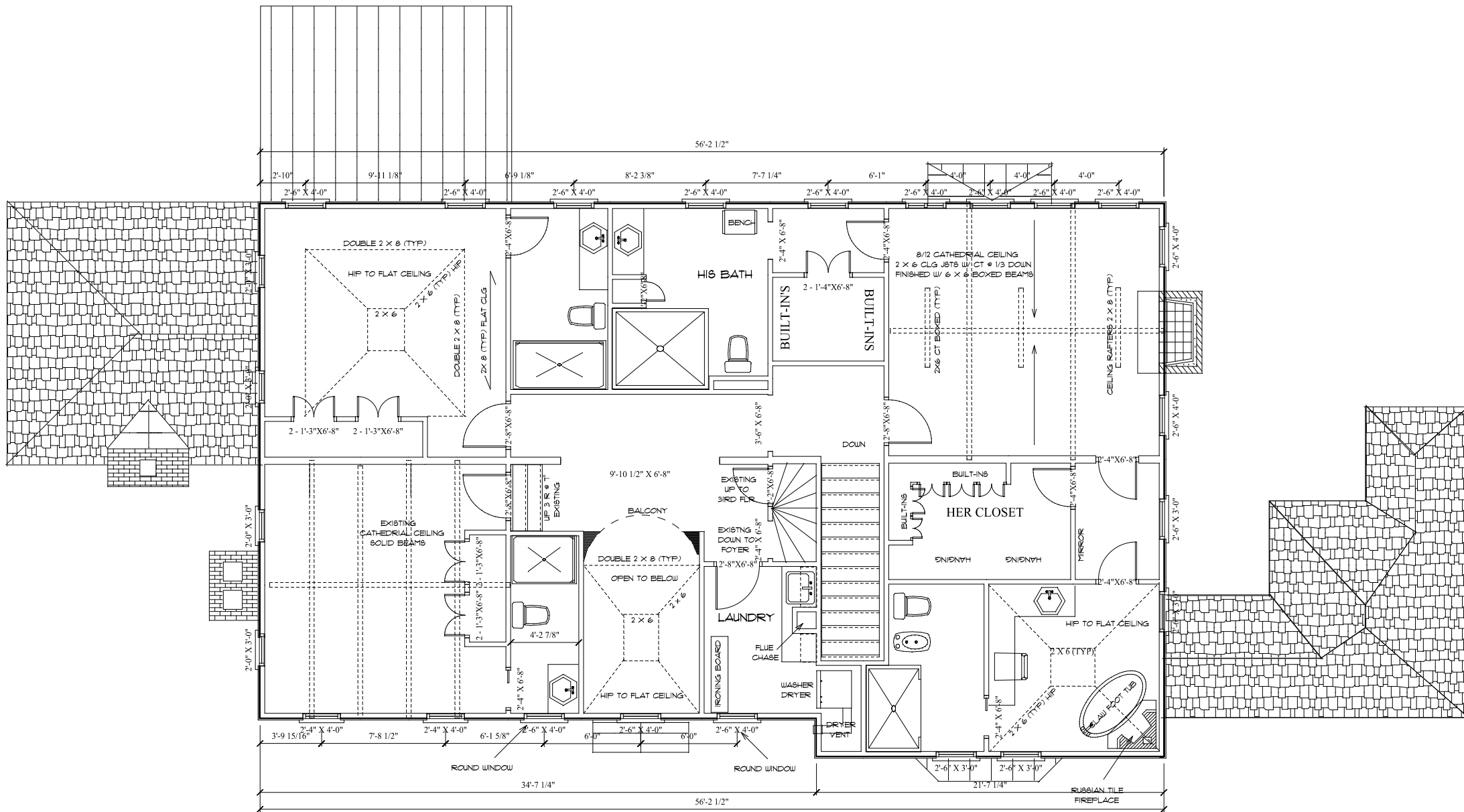
SECOND FLOOR PLAN Scale 1/8" = 1'-0"
